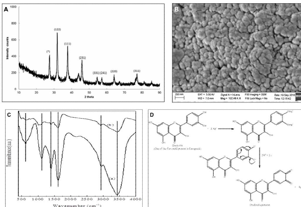
Fig. 2(A). XRD pattern of biosynthesized AgNPs using 1 ml of leaf extract and 2.25 mM \text{AgNO}_3 at 100^\circ\text{C} for a time duration of 2 hrs; (B) FESEM image of AgNPs; (C) FTIR spectra of (a) pure leaf extract, (b) Silver nanoparticles; (D) The possible mechanism for the formation of bio-reduced AgNPs.
