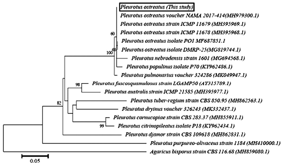
Fig. 3. Phylogenetic tree showing the relationship between P. ostreatus used in this study (GenBank accession No. MT672600) with other fungi. The tree was constructed by maximum likelihood method based on Tamura and Nei (1993) integrated in the MEGA7.0 software (Kumar et al. 2016). The phylogenetic tree was tested with 1000 bootstrap replicates.
