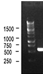
Fig. 2. Agarose gel electrophoresis of PCR product. The PCR product was electrophoresed in 0.8% agarose gel visualized under UV after staining with ethidium bromide. The bands in the left lane represent DNA size marker.
