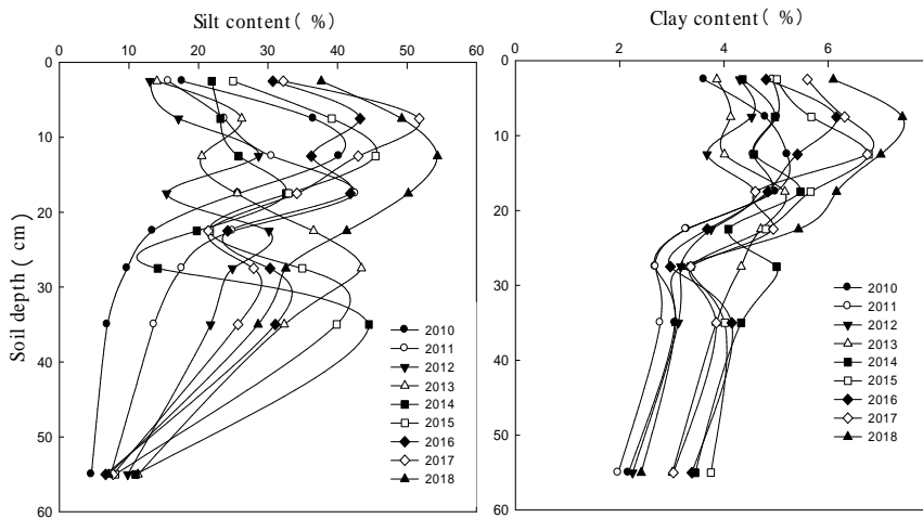
Fig. 4. Migration characteristics of clay and silt in 1 : 1 compound soil.
