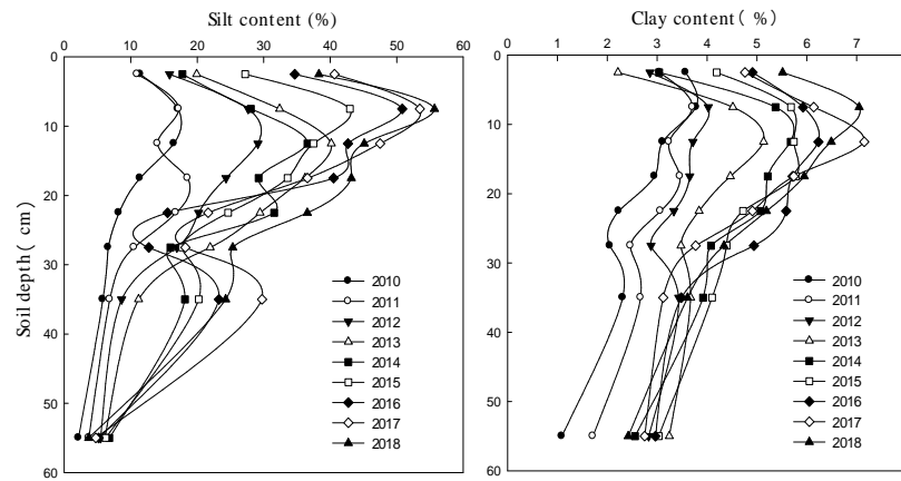
Fig. 5. Migration characteristics of clay and silt in 1 : 2 compound soil.
