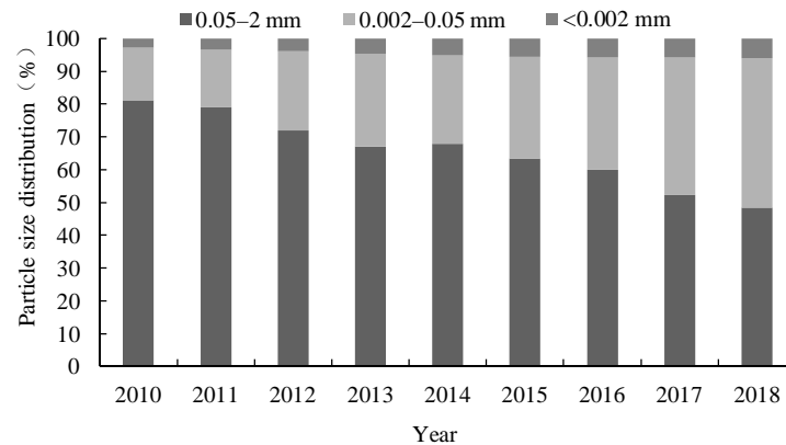
Fig. 2. Particle size composition of 1:2 compound soil under different planting years.
