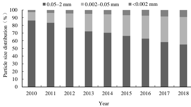
Fig. 3. Particle size composition of 1:5 compound soil under different planting years.
