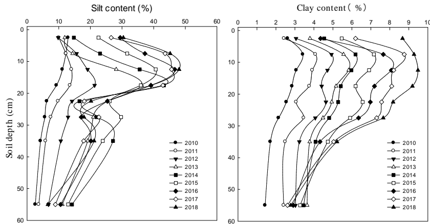
Fig. 6. Migration characteristics of clay and silt in 1 : 5 compound soil.
