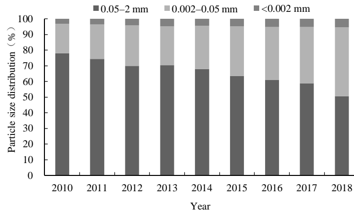
Fig. 1. Particle size composition of 1:1 compound soil under different planting years.
