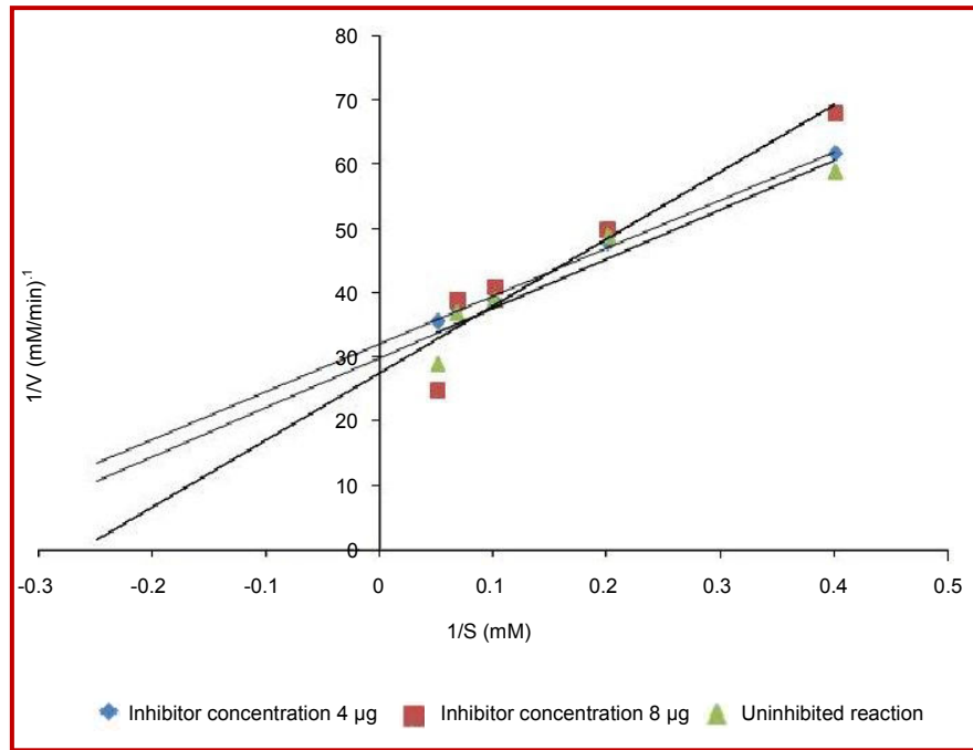
Figure 2 : Lineweaver-Burk plot of S. cerevisiae \alpha -glucosidase and PNPG with 4 \mu\text{g}/\text{mL} and 8 \mu\text{g}/\text{mL} of Aegle marmelos extracts
