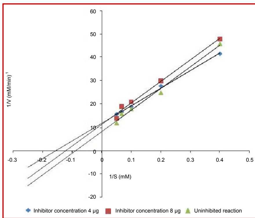
Figure 1 : Lineweaver-Burk plot of S. cerevisiae \alpha -glucosidase and PNPG with 4 \mu\text{g}/\text{mL} and 8 \mu\text{g}/\text{mL} of Citrullus colocynthis extract
