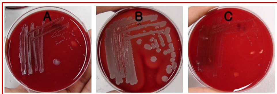
Figure 3: Hemolytic phenomenon test. (A) Test strain: Lactobacillus plantarum YML009. (B) \beta control: Streptococcus agalactiae KCCM 40417. (C) \alpha Control: Lactobacillus paracasei KCTC 3510
