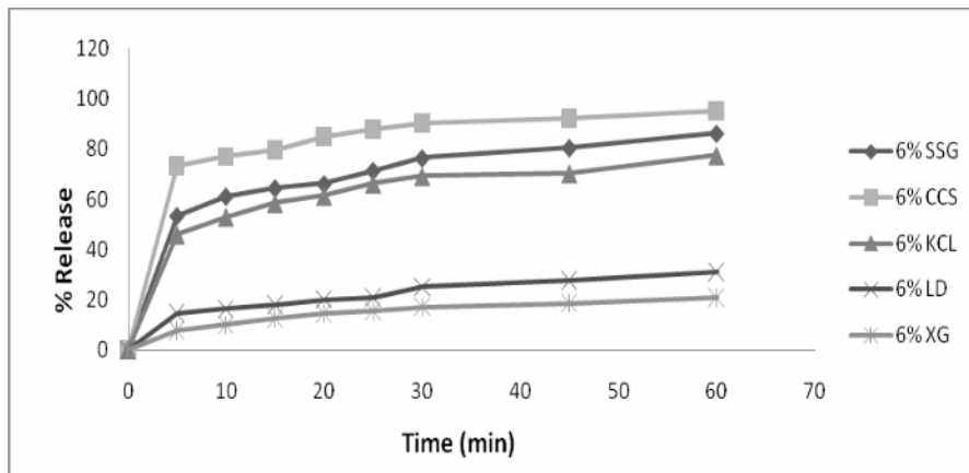
Figure 3. Zero order curve for F-2, F-5, F-8, F-11 and F-14.
