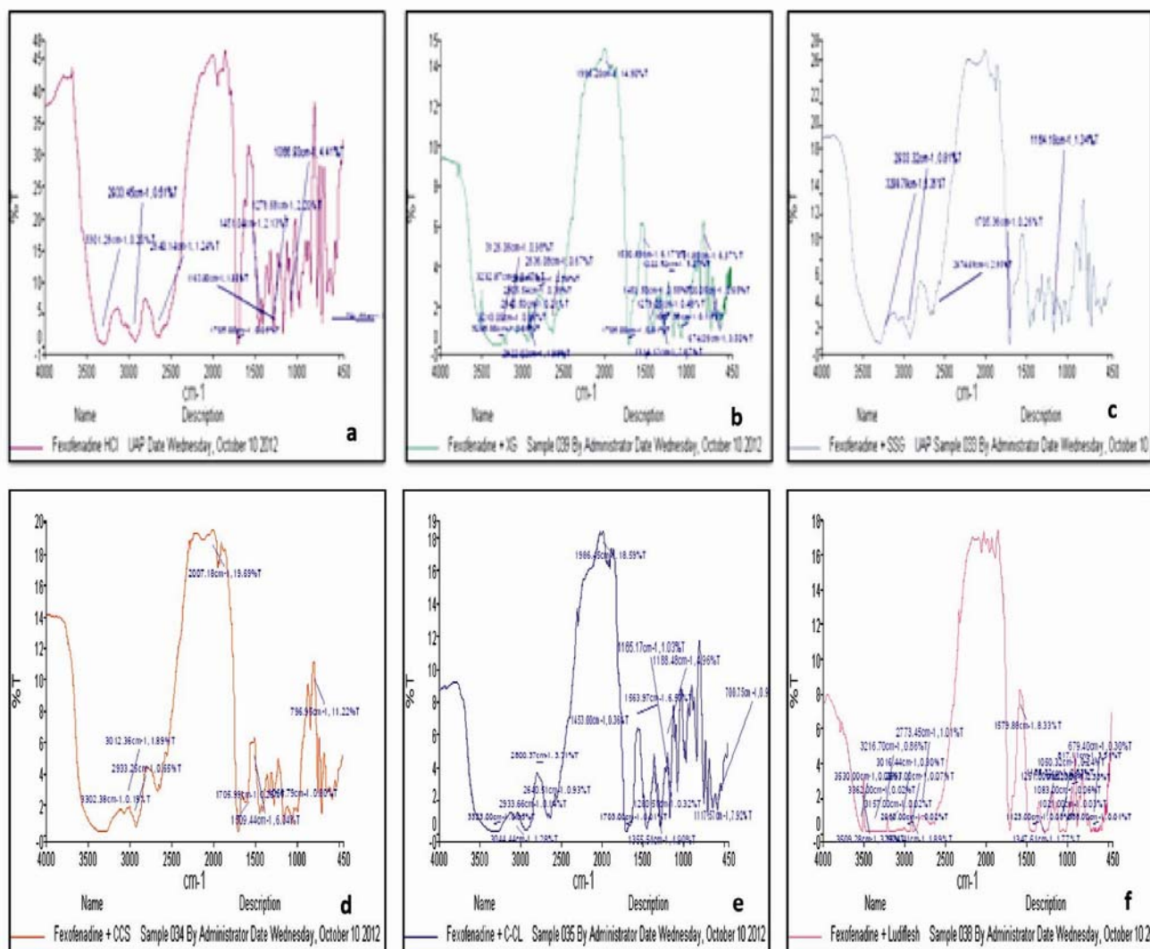
Figure 6. a, b, c, d, e and f represent IR spectra of pure FFN (Drug), FFN formulation with 8% XG, FFN formulation with 8% SSG, FFN formulation with 8% CCS, FFN formulation with 8% KCL and FFN formulation with 8% Ludiflash, respectively.
