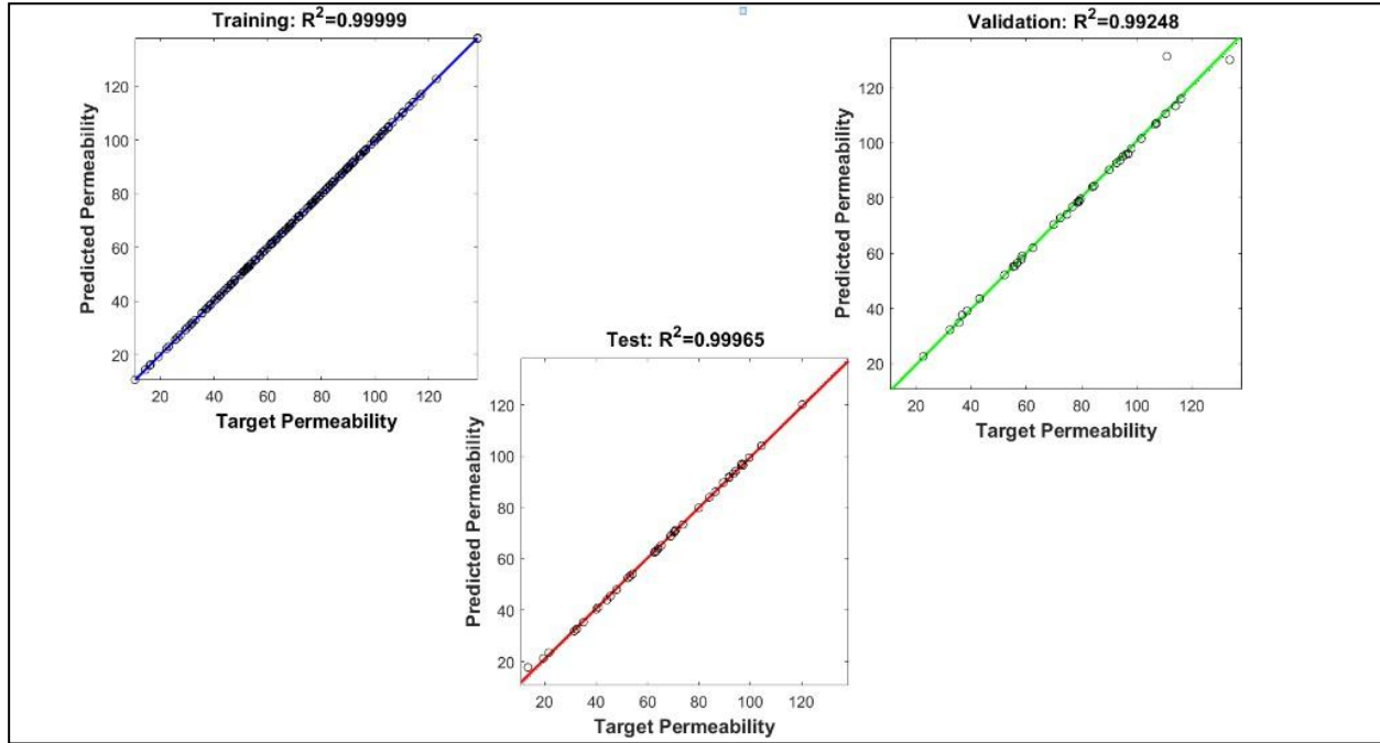
Figure 2: ANN model performance of training, testing and validation with Levenberg- Marquardt algorithm.
