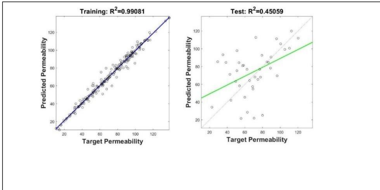
Figure 3: ANN model performance of training and testing for Bayesian regularization algorithm.
