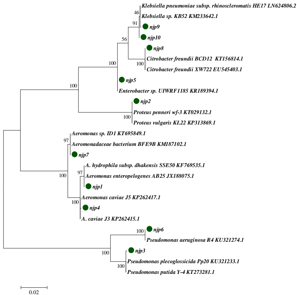
Fig. 3. The neighbor-joining (NJ) phylogenetic tree based on partial 16S rRNA gene sequences conducted using MEGA v.6. The evolutionary distances were compared by Maximum Likelihood method, bootstrap 1000 replicates. Green circles indicate position of the studied strains.
