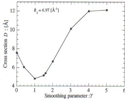
Fig. 6. Variation of step cross section with smoothing parameter for a particular beam energy corresponding to k_i = 6.97 \text{ \AA}^{-1} .
