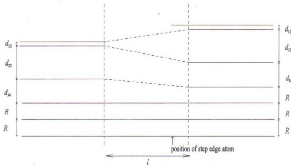
Fig 1. A schematic diagram showing the seven upper most layers of an isolated up step of Cu(001). The first two layers are contracted, the second and third layers expanded, third and fourth layers are also expanded but d_{34} < d_{23} (inter layer spacings) and starting from the fifth layer the layers are in their normal bulk positions with regular spacing R=1.803 \text{ \AA} .
