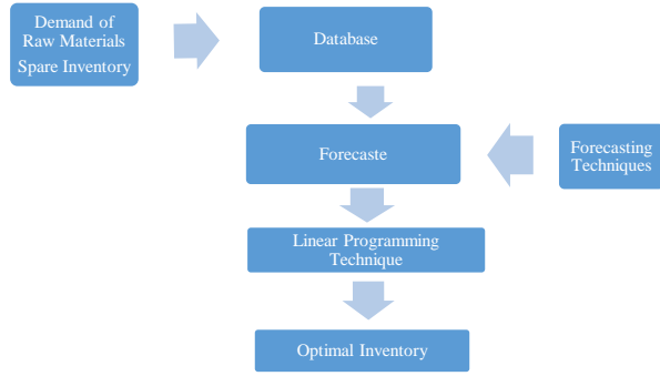
Fig. 1. Flowchart of the Research Model
