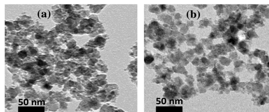
Figure 2: TEM micrographs in (a) Bare and (b) Chitosan-coated CoFe_2O_4 nanoparticles.
