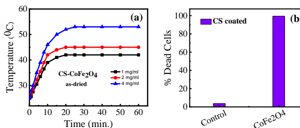
Figure 5: (a) RF induction heating properties of the chitosan-coated CoFe_2O_4 at different concentrations (b) Necrosis of 9L tumor cells by RF induction heating for 30 min without nanoparticle (control) and with chitosan-coated CoFe_2O_4 nanoparticle at the 2 mg/ml concentration in PBS by applying ( H = 20 mT and f = 342 kHz ).
