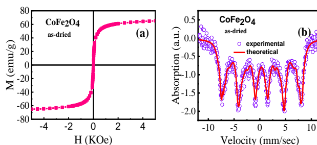
Figure 3: (a) MH hysteresis loop and (b) Mössbauer spectroscopy of CoFe_2O_4 nanoparticles in the as-dried condition at room temperature.
