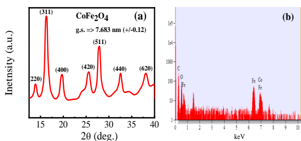
Figure 1: (a) XRD pattern of CoFe_2O_4 nanoparticles in the as-dried condition at the room temperature and (b) EDX spectrum of CoFe_2O_4 nanoparticles in the as-dried condition with liquid form.
