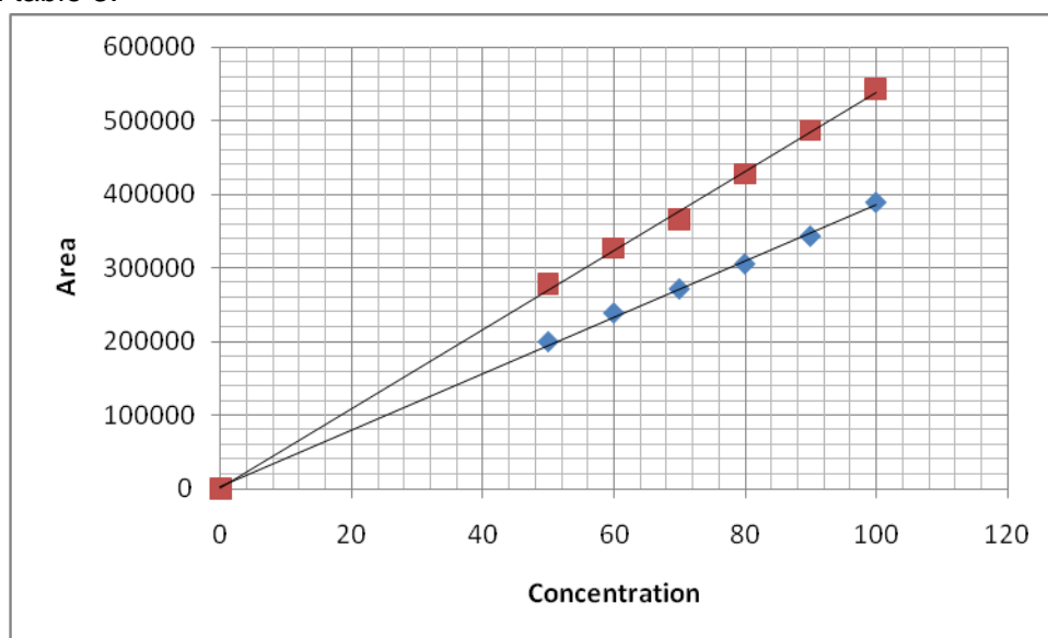
Graph 1: Calibration Plot for Ezetimibe and Simvastatin
