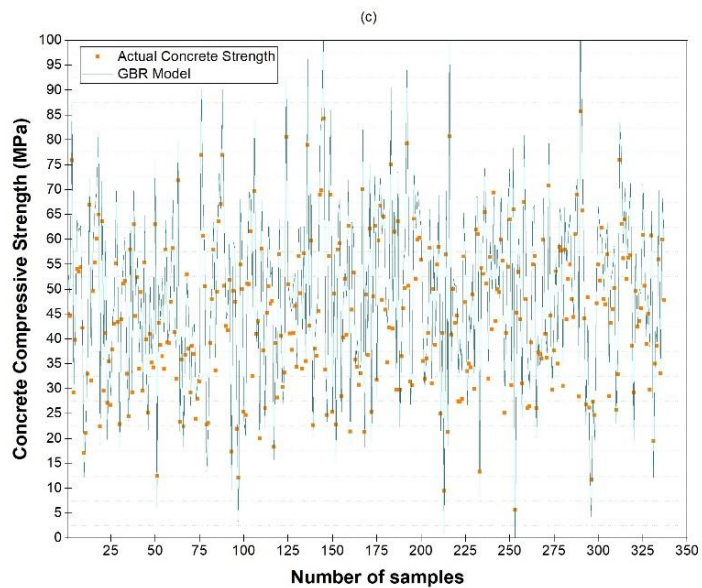
Figure 6: Comparison of measured compressive strength with predictions for training dataset; (a) ANN model, (b) RF model, and (c) GBR model
