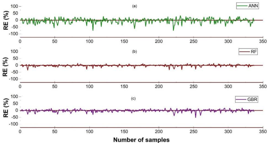
Figure 7: Relative error (RE) plots for the training dataset samples; (a) ANN model, (b) RF model, and (c) GBR model
