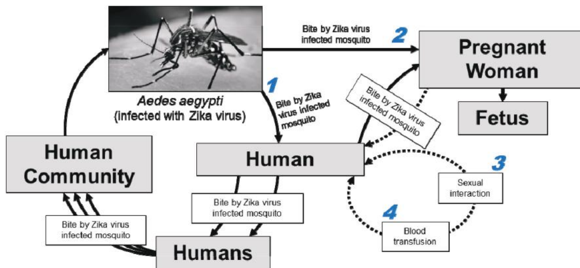
Figure 2. Transmission of Zika virus. (1) Infected mosquito (particularly female A. aegypti ) may bite a healthy human. The Zika infected human may act as a source of infection for other humans in the community. (2) Infected pregnant woman may act as a source for Zika virus transmission to her fetus. (3) Human to human transmission may occur by sexual interaction between male and female. (4) Blood transfusion may cause Zika virus transmission from one human to another.
