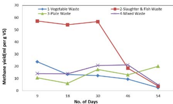
Fig. 4 Specific average methane yield
