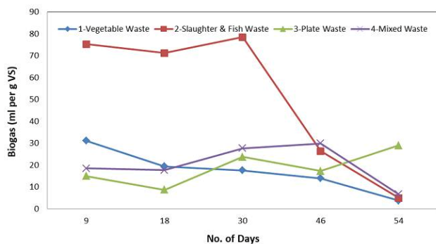
Fig. 2 Specific biogas production from selected substrates during the batch assay
