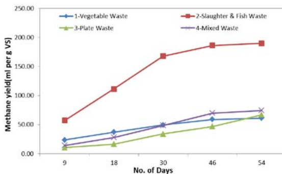
Fig. 5 Cumulative bio-methane production from selected substrates
