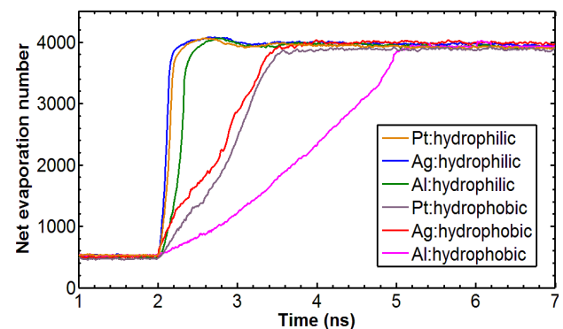
Fig.12. Time variation of net evaporation number
