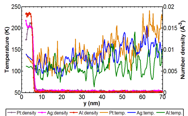
Fig.10. Spatial distribution of temperature and density of argon for hydrophobic Pt, Ag and Al-surface at 2.5ns.
