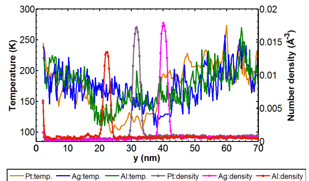
Fig. 9. Spatial distribution of temperature and density of argon for hydrophilic Pt, Ag, and Al-surface at 2.5 ns.
