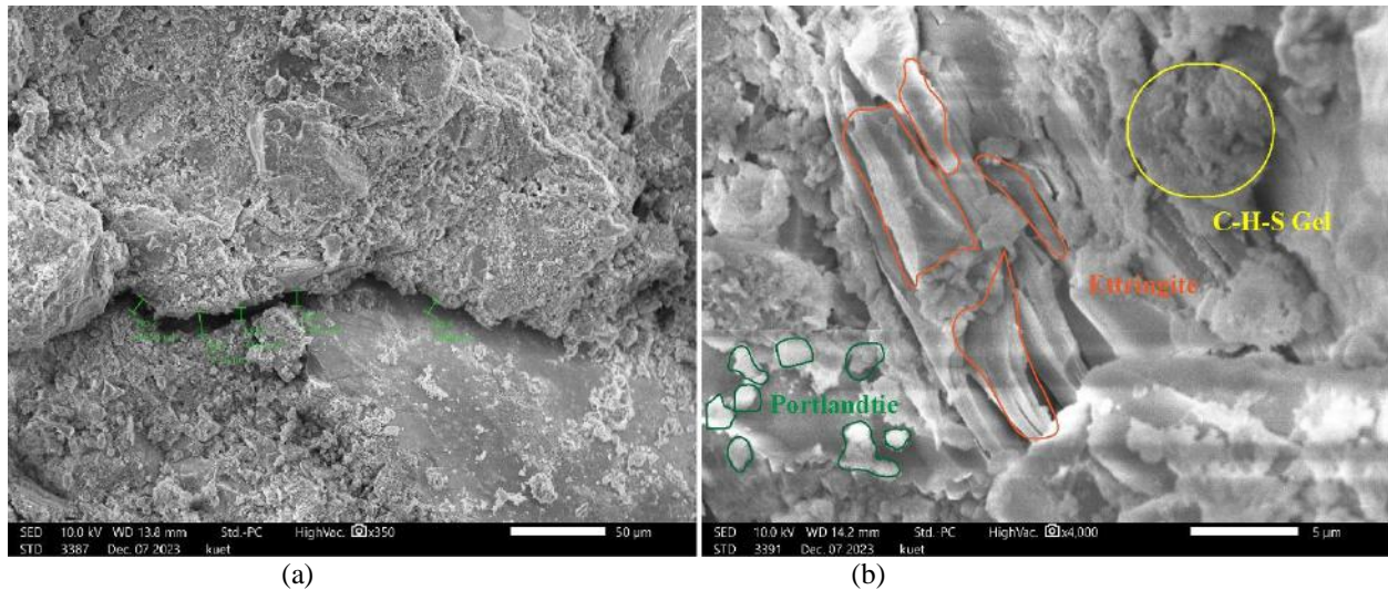
Figure 4: SEM images of Microstructure of Ordinary New Concrete interface (a) New Interfacial Transition Zone (ITZ), (b) Ordinary New concrete showing Calcium Silicate Hydrate (C-S-H) gel, Portlandite (C-H) crystals and Ettringite (Aft) crystals.
