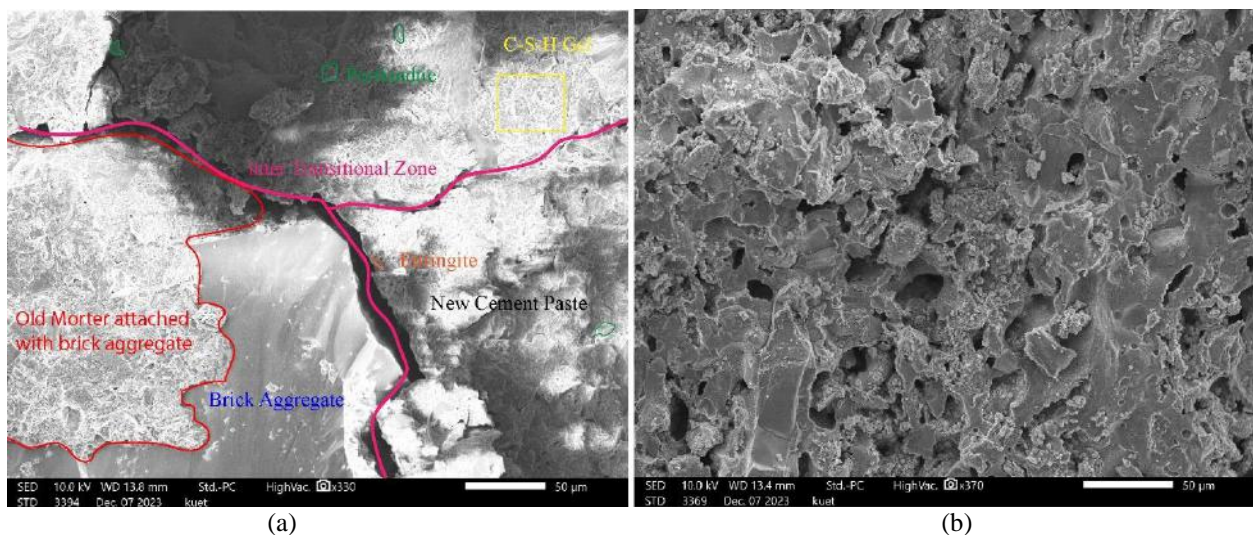
Figure 5: SEM images of Microstructure of Recycled Concrete interface (a) Interfacial Transition Zone (ITZ), (b) Pores or voids in Recycled Concrete Surface
