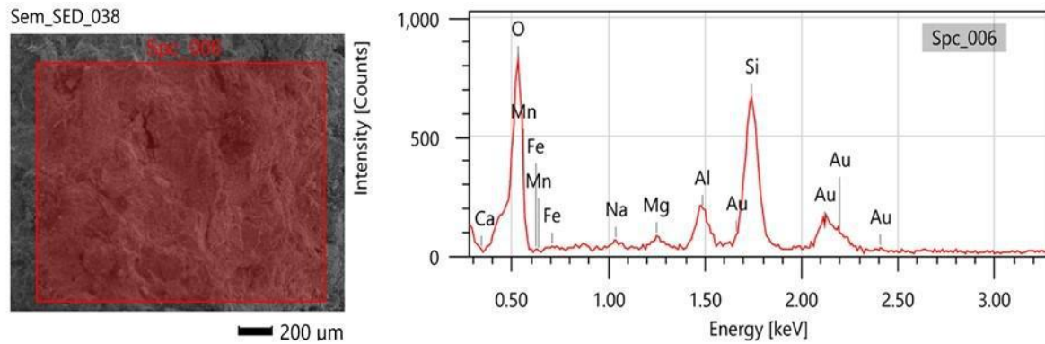
Figure 9: SEM micrographs of recycled concrete with EDS pattern
