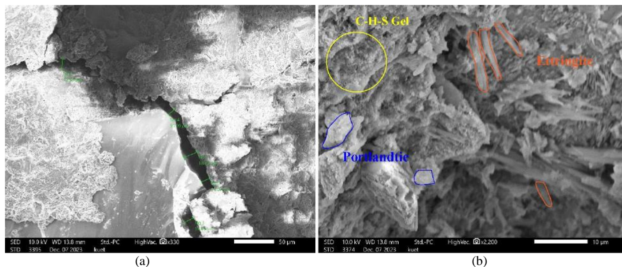
Figure 6: SEM images of the Microstructure of Recycled Concrete interface (a) Interfacial Transition Zone (ITZ)(b) Recycled Concrete showing Calcium Silicate Hydrate (C-S-H) gel, Portlandite (C-H) crystals and Ettringite (Aft) crystals.
