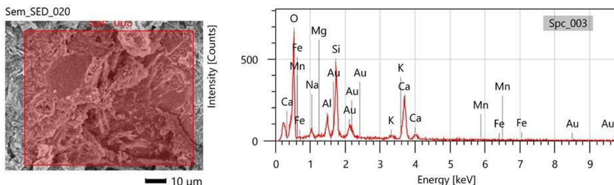
Figure 7: SEM micrographs of old concrete with EDS pattern
