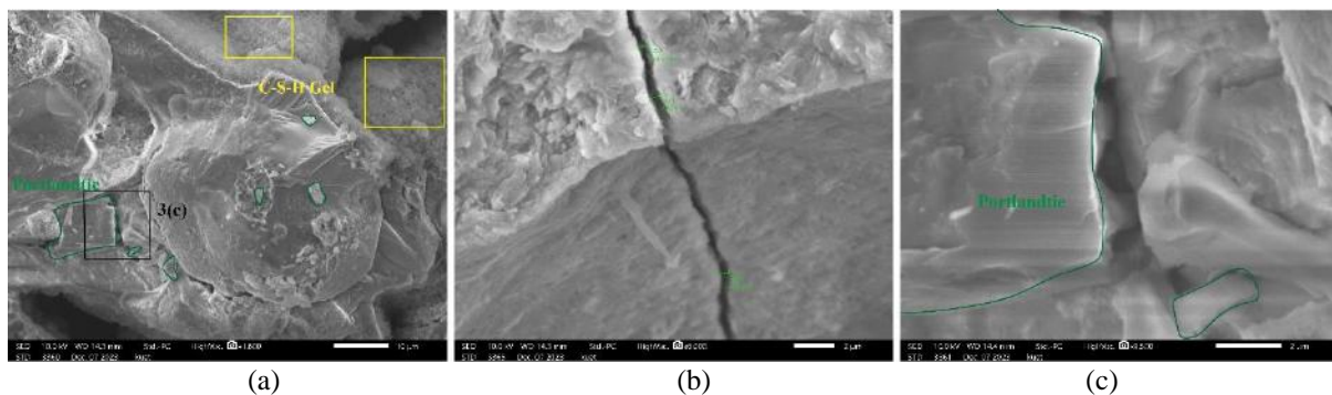
Figure 3: SEM images of (a) Microstructure of Old Concrete interface showing Calcium Silicate Hydrate (C-S-H) gel, Portlandite (C-H) crystals (b) Old Interfacial Transition Zone (ITZ), (c) Old concrete showing Portlandite (C-H) crystals.
