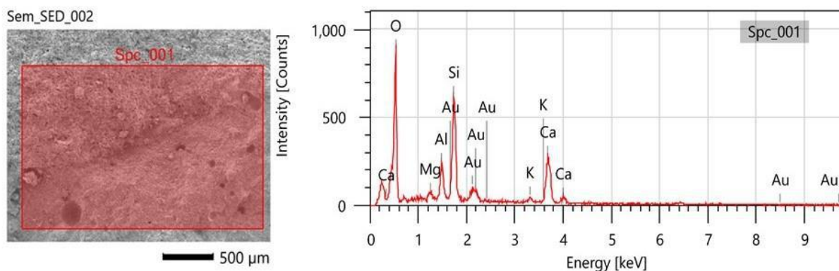
Figure 8: SEM micrographs of ordinary new concrete with EDS pattern
