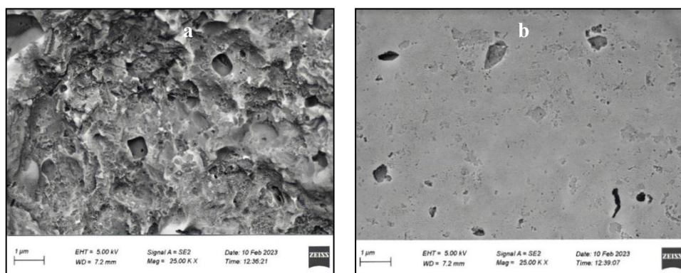
Figure 7: Pure Tamarindus indica leaves adsorbent (a) dye load Tamarindus indica leaves adsorbent (b)
