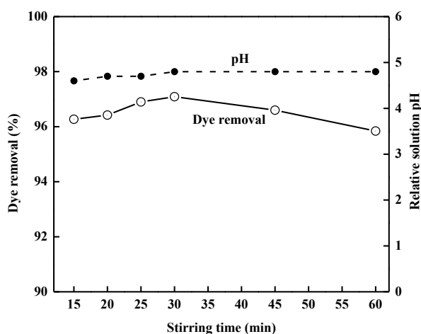
Figure 4: Effect of stirring time on dye removal efficiency from wastewater
