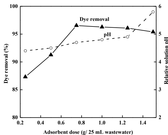
Figure 3: Effect of adsorbent doses on dye removal efficiency from wastewater
