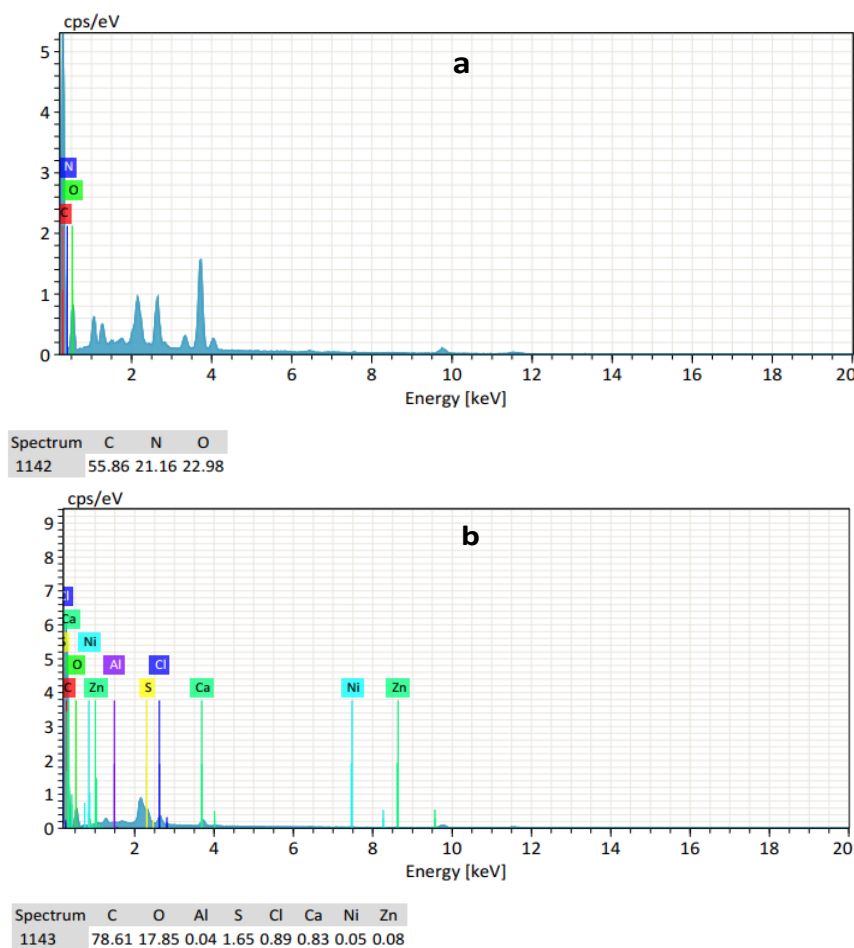
Figure 8: EDS spectrum of pure Tamarindus indica leaves adsorbent (a) dye-loaded Tamarindus indica leaves adsorbent (b)
