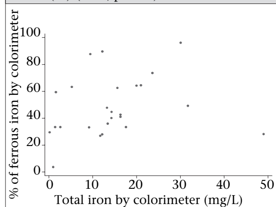
Fig. 1. Ferrous iron as a percentage of total iron defined by the colorimeter [percent ferrous iron = 435.6 + \text{total iron (mg/L)} * (-0.003, p > 0.99) + \text{pH} * (5.5, p = 0.73) + \text{temperature (°C)} * (-16.0, p = 0.11) ]
