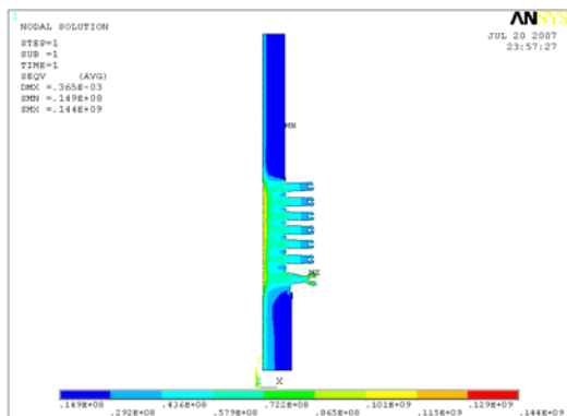
Fig 7. Von-Mises Stress
