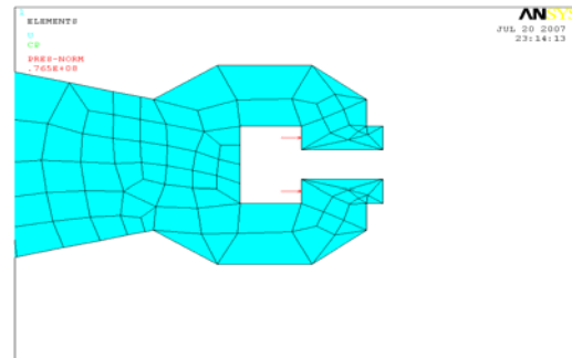
Fig 4. Pressure applied at the Rotor Groove
