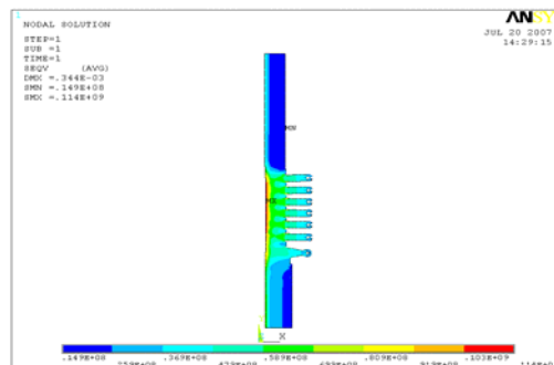
Fig 10. Von-Mises Stress
