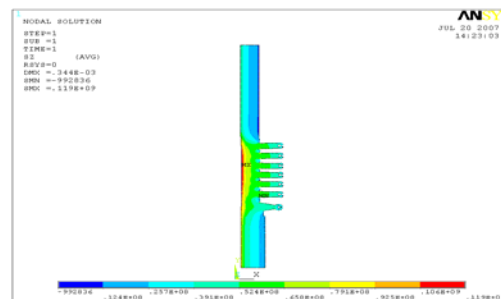
Fig 9. Max Hoop Stress
