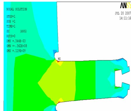
Fig 8. Max Radial Stress
