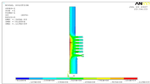
Fig 6. Max Hoop Stress
