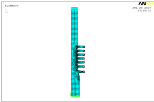
Fig 2. Boundary Conditions
