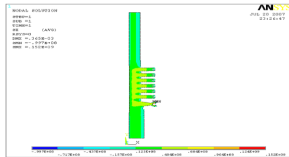
Fig 5. Max Radial Stress
