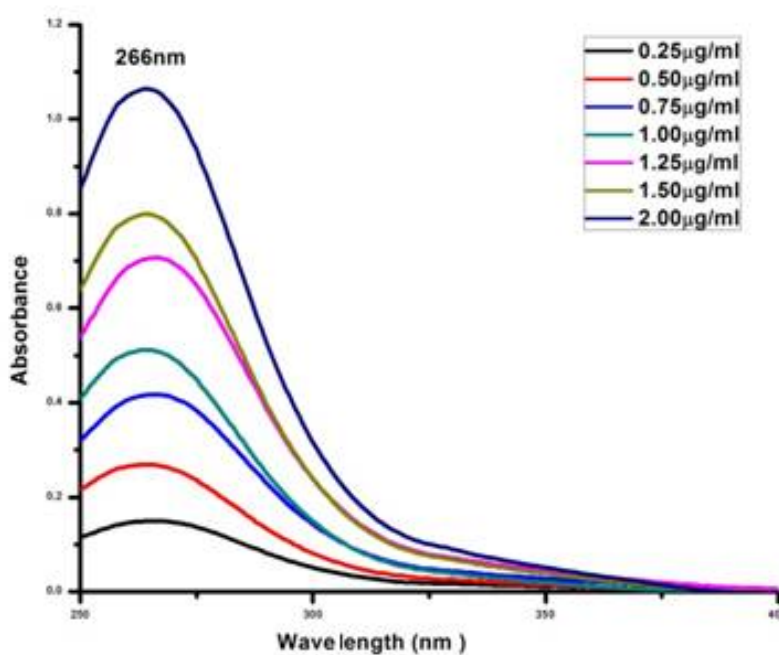
Figure 2. Absorption spectra of PTC in 0.01M HCl at different concentrations (method B)
