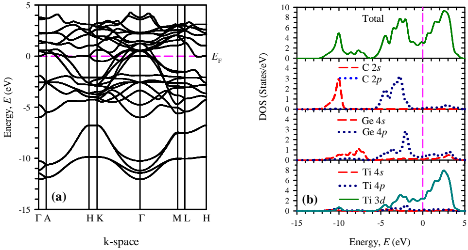
Fig. 3(a). Band structure and (b) total and partial density of states for \text{Ti}_2\text{GeC} at zero pressure.
