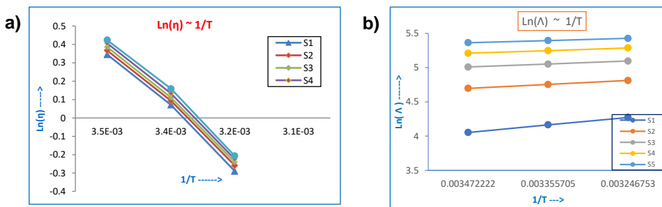
Fig. 1. Variations of a) \ln(\eta) and b) \ln(\Lambda) with the inverse of temperature for all solutions.
