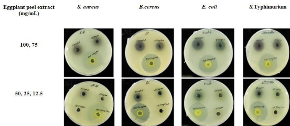
Fig. S2. Antibacterial effect of water-reconstituted eggplant peel extract using agar well diffusion assay.
