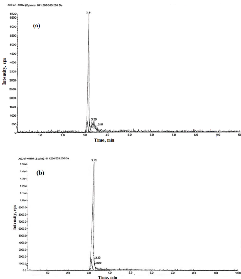
Fig. S1. LC-MS/MS chromatogram of a) Water-reconstituted eggplant peel extract and b) Delphinidin-3-rutinoside standard.
