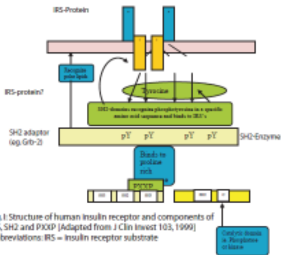
Figure-I: Structure of human insulin receptor and components of IRS, SH2 and PXXP [Adapted from J Clin Invest 103, 1999] Abbreviations: IRS=insulin receptor substrate.
