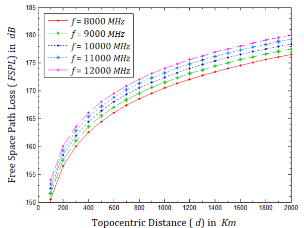
Figure 3: Behavior of FSPL over the variation of Topocentric distance (distance between Earth station & Satellite) ( d ) in range of X-band frequency ( f ) (8 GHz to 12 GHz) (Mahmud & Khan, 2009; Song, & Schnieder, 2019)
